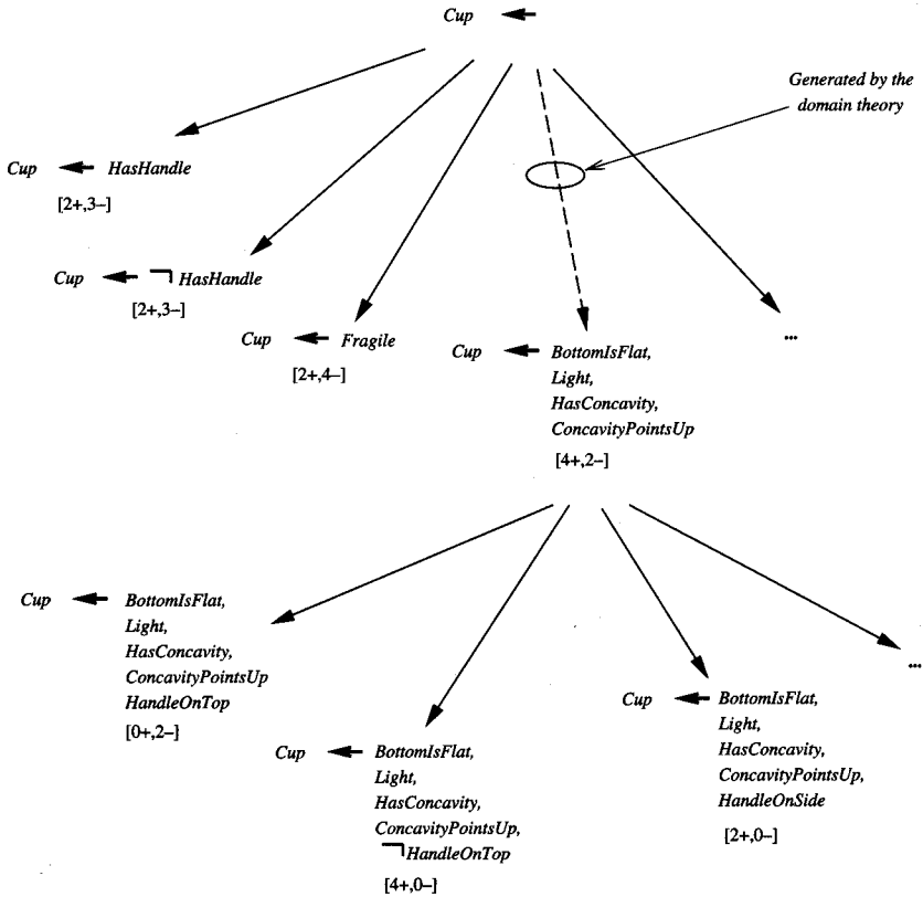
FIGURE 12.8 Hypothesis space search in FOCL. To learn a single rule, FOCL searches from general to increasingly specific hypotheses. Two kinds of operators generate specializations of the current hypothesis. One kind adds a single new literal (solid lines in the figure). A second kind of operator specializes the rule by adding a set of literals that constitute logically sufficient conditions for the target concept, according to the domain theory (dashed lines in the figure). FOCL selects among all these candidate specializations, based on their performance over the data. Therefore, imperfect domain theories will impact the hypothesis only if the evidence supports the theory. This example is based on the same training data and domain theory as the earlier KBANN example.
